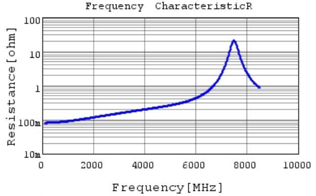
GCQ1555C1H9R0WB01 R DC0V, 25degC
