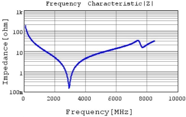
GCQ1555C1H9R0WB01 |Z| DC0V, 25degC
