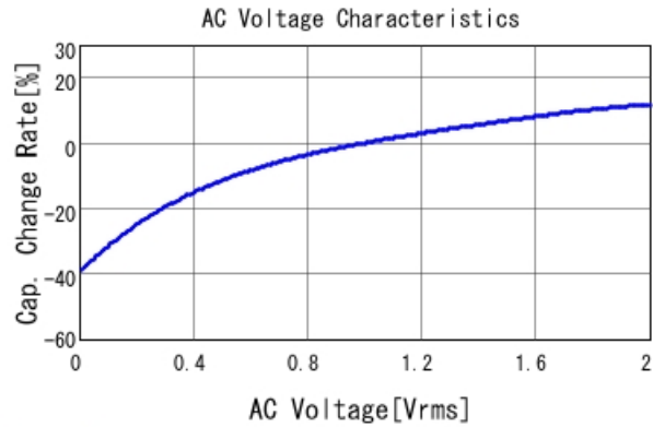
GCH188R71C105KE01 C-AC Voltage capchange, DCOV, 25
