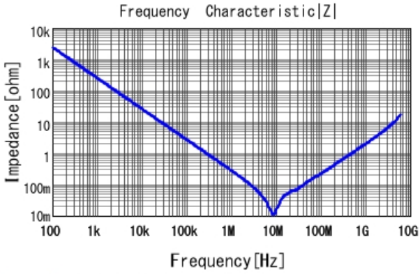
GCH188R71C105KE01 |Z| DCOV, 25degC
