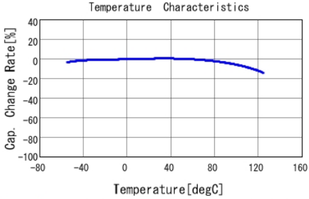
GCH188R71C105KE01 C-Temp. capchange, DC0.0V, AC1.C
