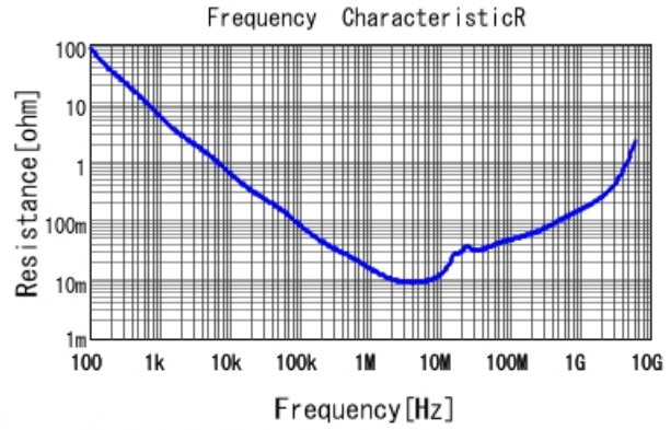
GCH188R71C105KE01 R DCOV, 25degC
