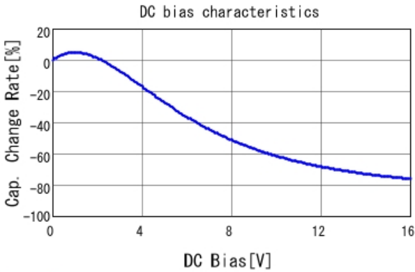
GCH188R71C105KE01 C-DC bias capchange, 25.0degC, A
