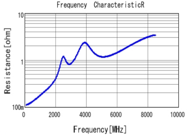
■ GRM1552C1E560JA01 R DCOV, 20degC
