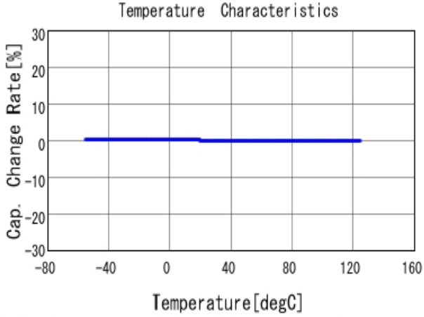
■ GRM1552C1E560JA01 C-Temp. capchange, DCOV, AC1Vrms
