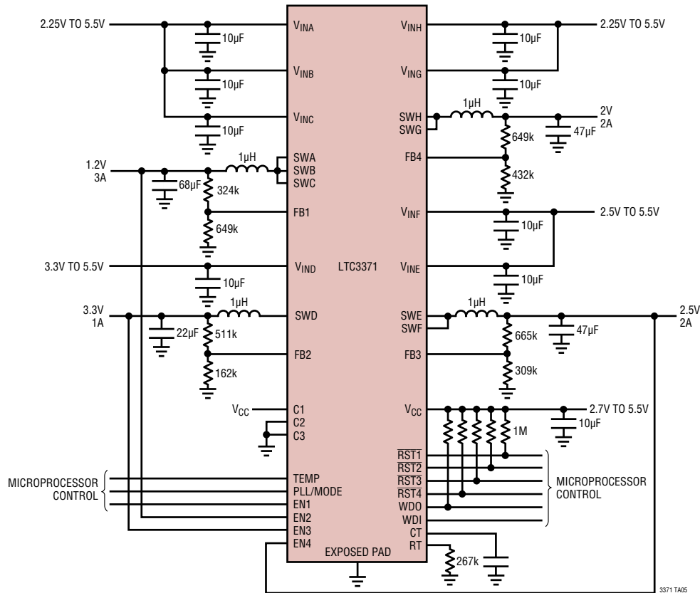
Combined Bucks with 3MHz Switching Frequency and Sequenced Power Up
