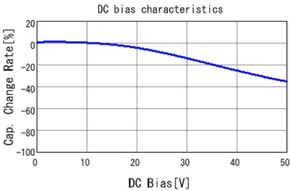
■ GCJ188R71H393KA12 C-DC bias capchange, 25.0degC, AC1.
