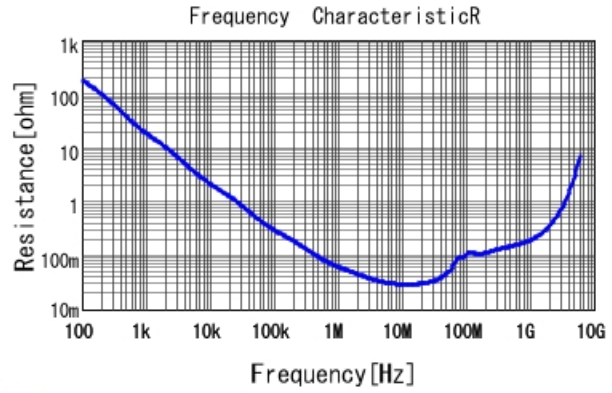
■ GCJ188R71H393KA12 R DC0V, 25degC
