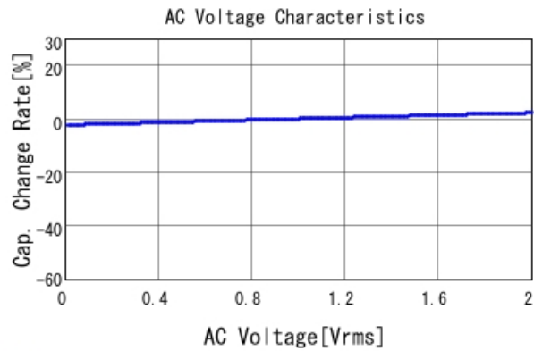
■ GCJ188R71H393KA12 C-AC Voltage capchange, DC0V, 25.0d
