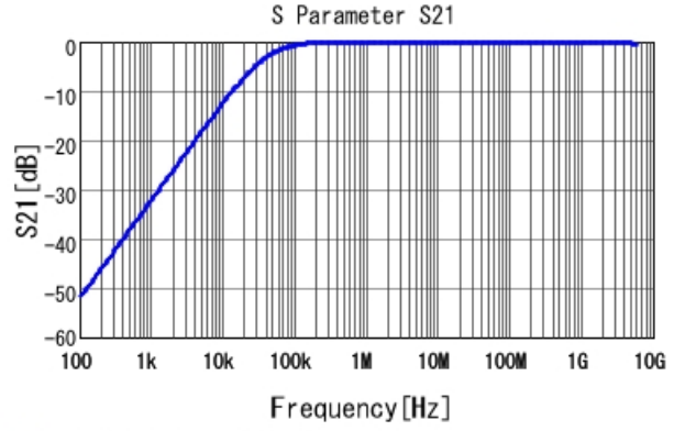
■ GCJ188R71H393KA12 S21 DCOV, 25degC
