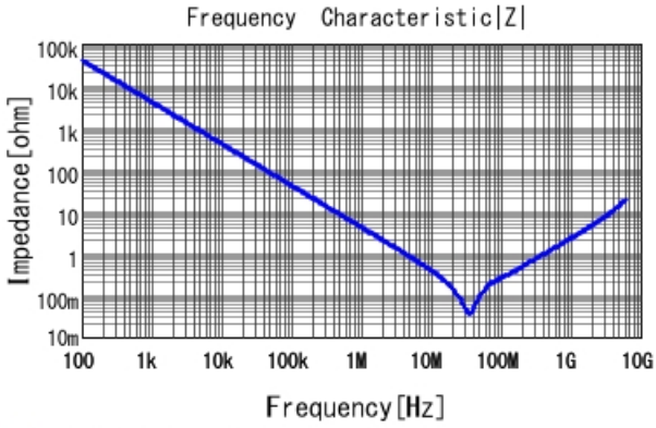
■ GCJ188R71H393KA12 |Z| DC0V, 25degC
