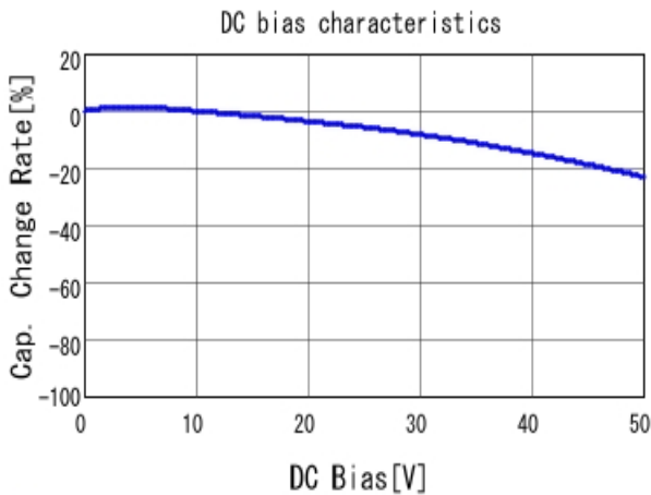
■ GRM155B11H331KA01 C-DC bias capchange, 20.0degC, AC1.
