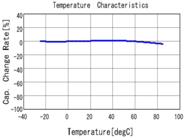
■ GRM155B11H331KA01 C-Temp. capchange, DCO. 0V, AC1.0Vrm
