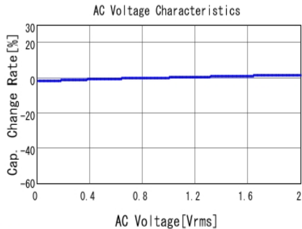
■ GRM155B11H331KA01 C-AC Voltage capchange, DCOV, 20.0d
