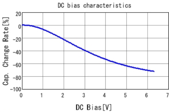
■ GRT155C80J475ME13 C-DC bias capchange, 25.0degC, AC0.
