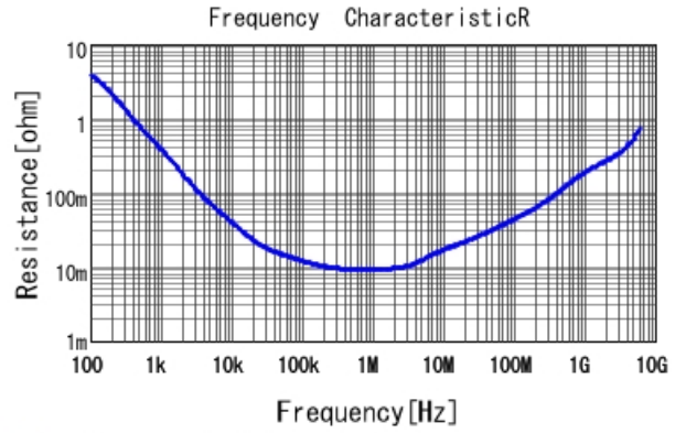
■ GRT155C80J475ME13 R DCOV, 25degC
