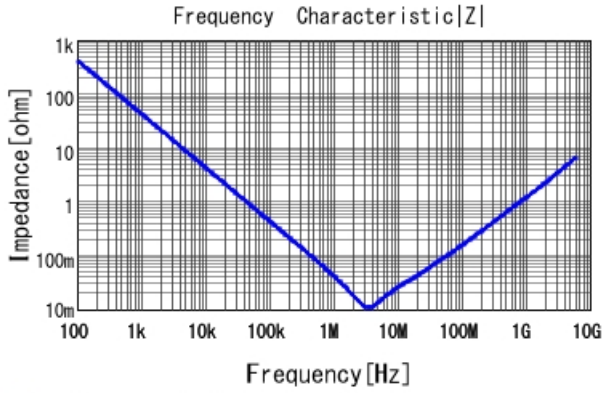
■ GRT155C80J475ME13 |Z| DCOV, 25degC
