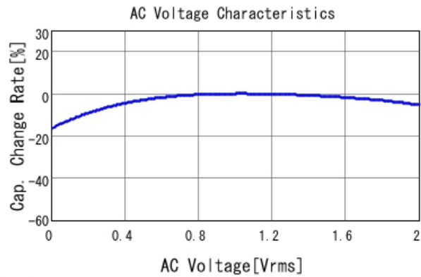
■ GRT155C80J475ME13 C-AC Voltage capchange, DCOV, 25.0d
