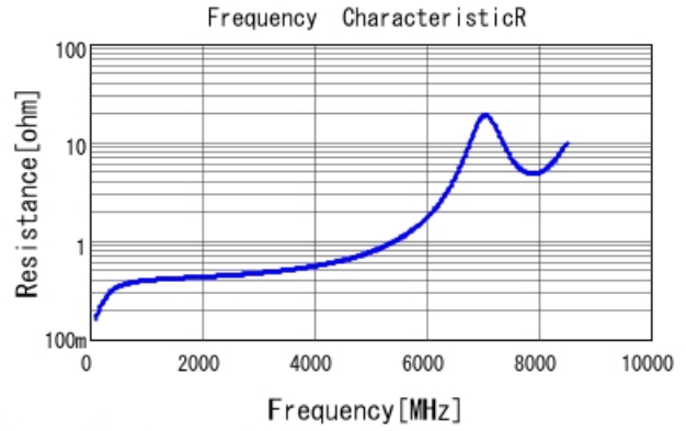
GRM1885C2A4R4CA01 R DCOV, 25degC
