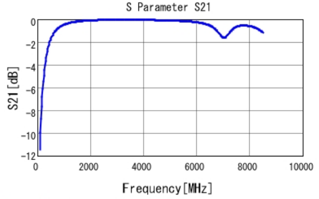
GRM1885C2A4R4CA01 S21 DC0V, 25degC
