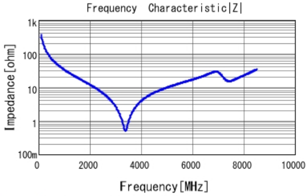
GRM1885C2A4R4CA01 |Z| DCOV, 25degC
