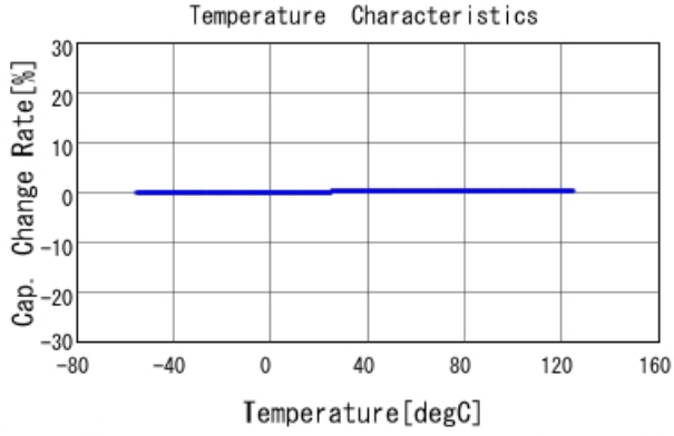
GRM1885C2A4R4CA01 C-Temp. capchange, DC0V, AC1Vrms
