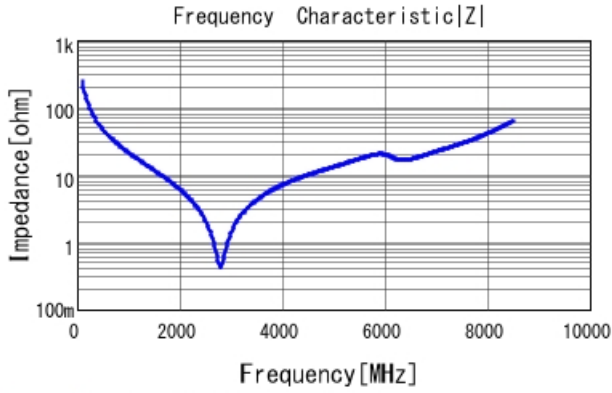
GRM1885C1H6R5WA01 |Z| DCOV, 25degC
