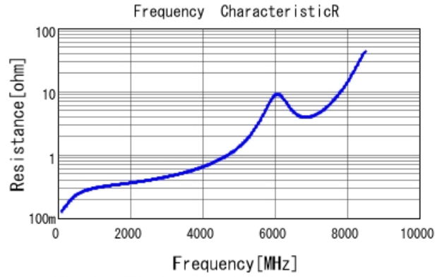
GRM1885C1H6R5WA01 R DCOV, 25degC
