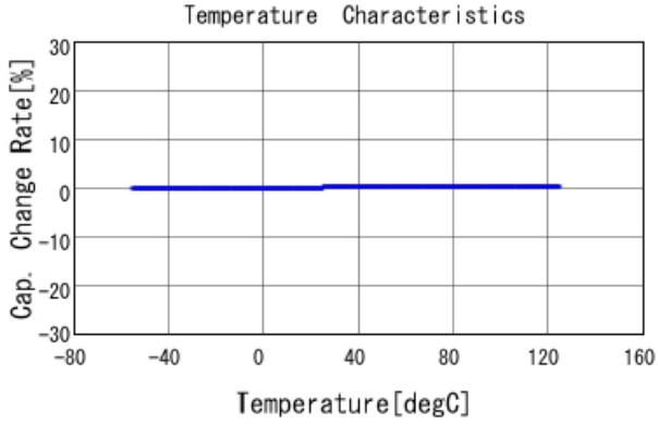
GRM1885C1H6R5WA01 C-Temp. capchange, DCOV, AC1Vrms
