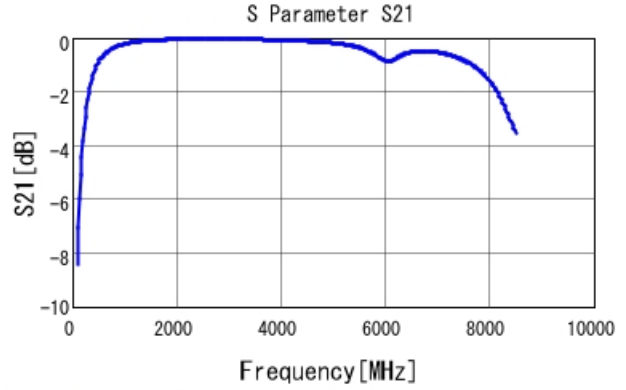
GRM1885C1H6R5WA01 S21 DCOV, 25degC
