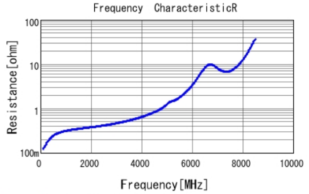
GRM1885C1H6R1WA01 R DCOV, 25degC
