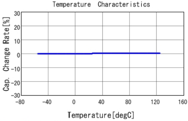
GRM1885C1H6R1WA01 C-Temp. capchange, DCOV, AC1Vrms
