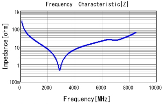
GRM1885C1H6R1WA01 |Z| DCOV, 25degC
