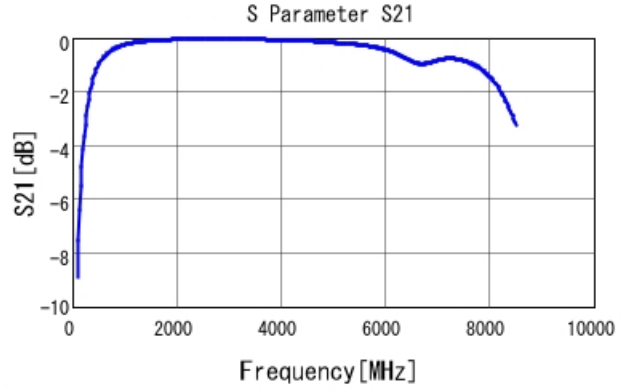
GRM1885C1H6R1WA01 S21 DCOV, 25degC
