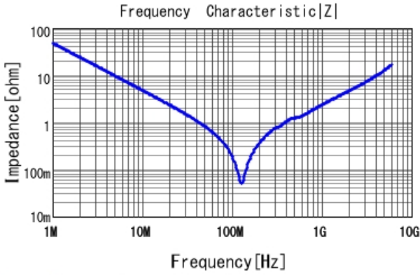
GRM1857U1H332JA44 |Z| DCOV, 25degC
