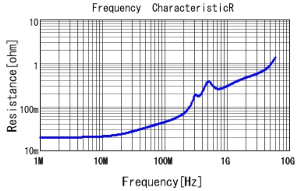
GRM1857U1H332JA44 R DCOV, 25degC
