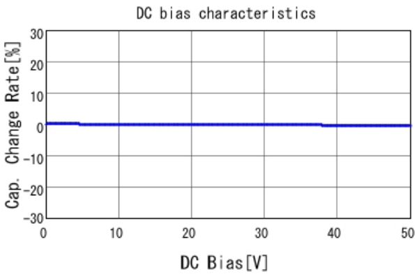
GRM1857U1H332JA44 C-DC bias capchange, 25.0degC, A
