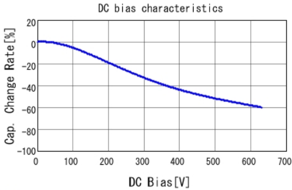
■ GC332DD72J333KX01 C-DC bias capchange, 25.0degC, AC1V
