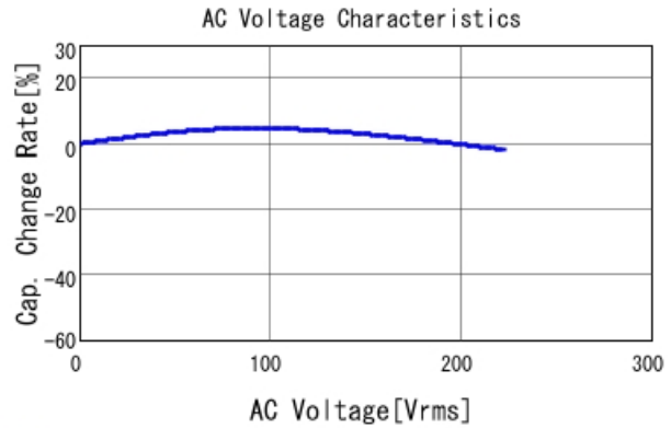
■ GC332DD72J333KX01 C-AC Voltage capchange, DC0V, 25.0d
