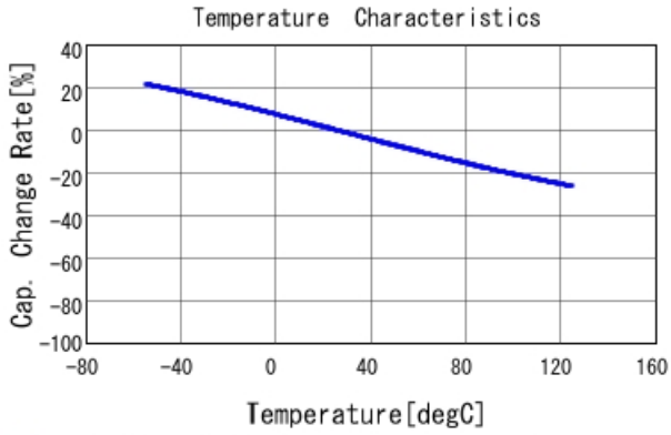
■ GC332DD72J333KX01 C-Temp. capchange, DCOV, AC1Vrms
