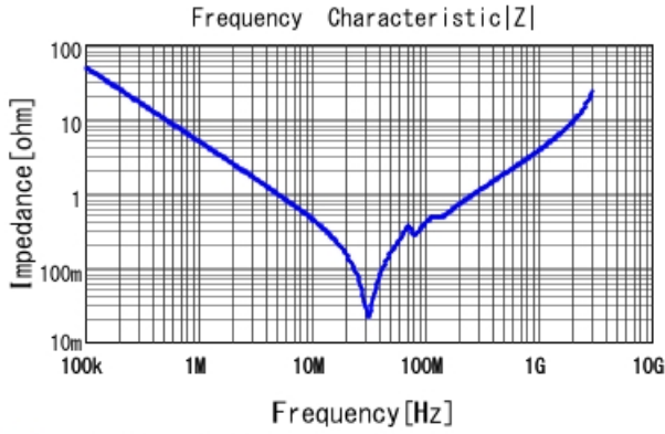
■ GC332DD72J333KX01 |Z| DC0V, 25degC
