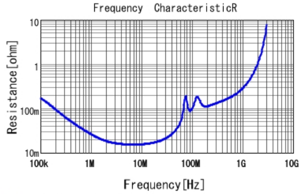
■ GC332DD72J333KX01 R DC0V, 25degC
