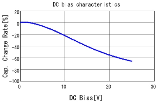
GRM32DC81E106KA12 C-DC bias capchange, 25.0degC, A
