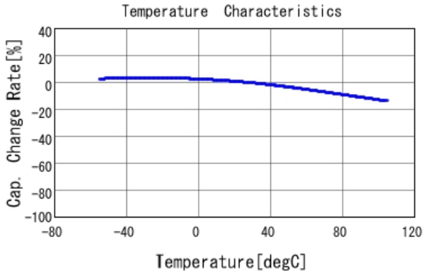
GRM32DC81E106KA12 C-Temp. capchange, DC0.0V, AC1.C
