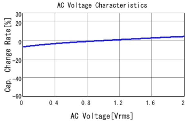
GRM32DC81E106KA12 C-AC Voltage capchange, DCOV, 25
