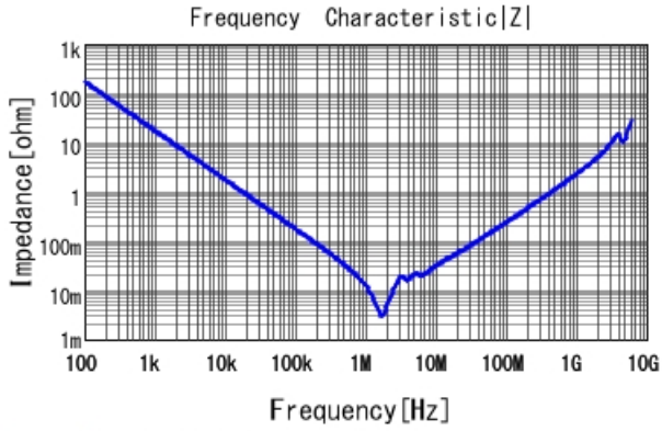
GRM32DC81E106KA12 |Z| DCOV, 25degC
