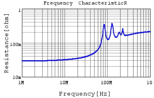
RCE5C1H223J1M1H03A R DC0V, 25degC
