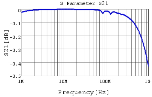
RCE5C1H223J1M1H03A S21 DC0V, 25degC
