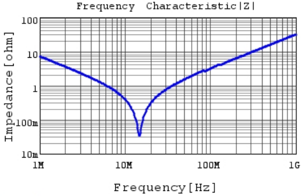
RCE5C1H223J1M1H03A |Z| DC0V, 25degC
