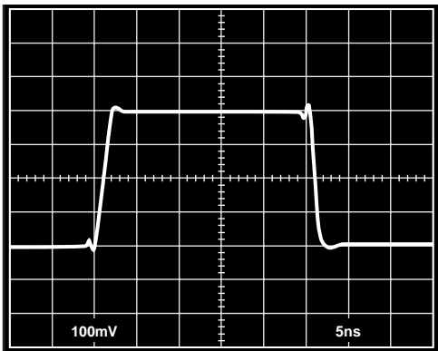
Figure 7. AD9631 Small Signal Transient Response; V_{OUT} = 400\text{ mV p-p} , G = +1 , R_F = 140\ \Omega
