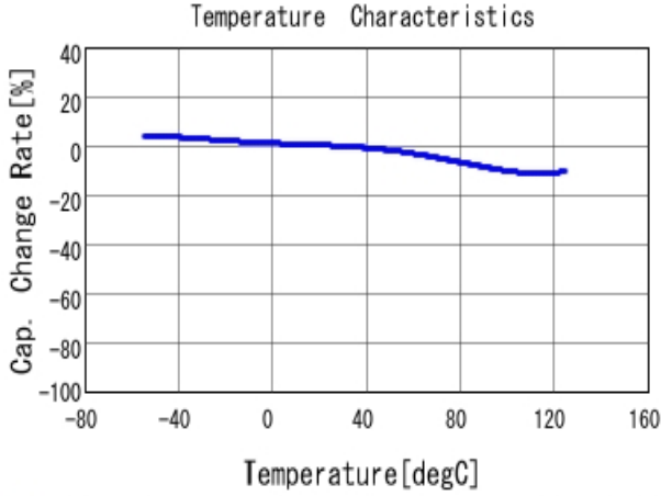
■ GRM155R71C153KA01 C-Temp. capchange, DCO. 0V, AC1.0V rm
