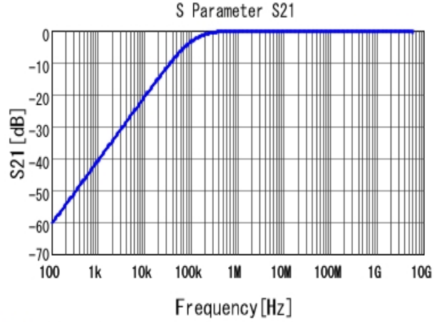
■ GRM155R71C153KA01 S21 DCOV, 25degC
