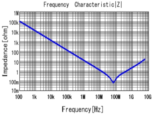
■ GRM155R71C153KA01 |Z| DCOV, 25degC
