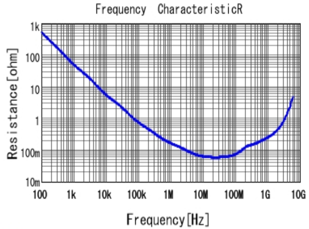
■ GRM155R71C153KA01 R DCOV, 25degC
