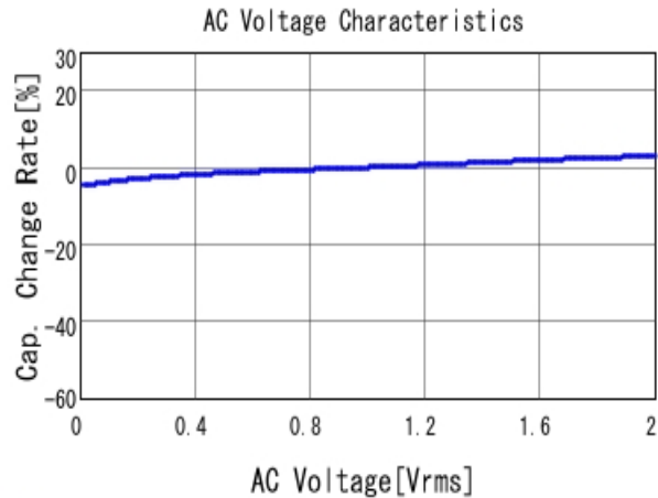
■ GRM155R71C153KA01 C-AC Voltage capchange, DCOV, 25.0d
