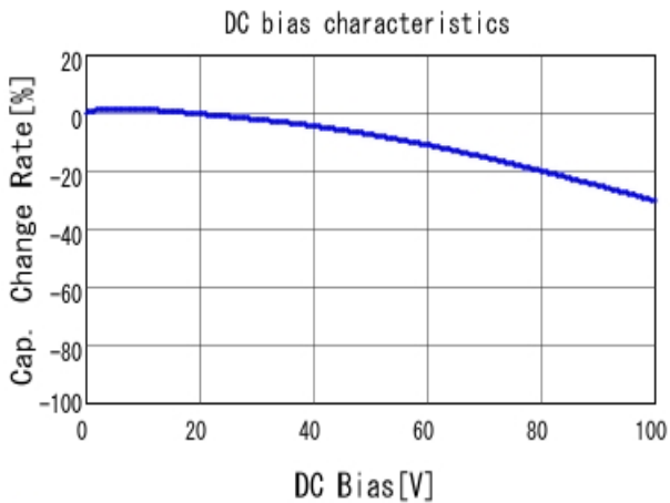
■ GRJ216R72A102KE01 C-DC bias capchange, 25.0degC, AC1.
