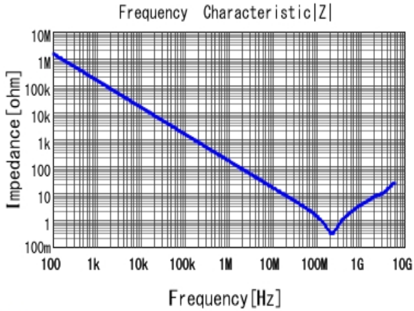
■ GRJ216R72A102KE01 |Z| DCOV, 25degC
