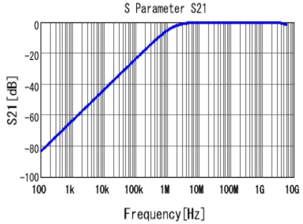
■ GRJ216R72A102KE01 S21 DC0V, 25degC
