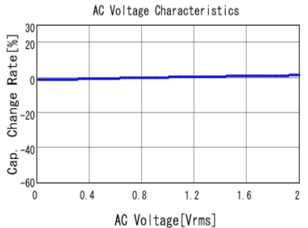
■ GRJ216R72A102KE01 C-AC Voltage capchange, DCOV, 25.0d
