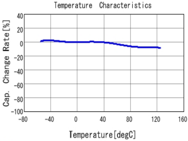
■ GRJ216R72A102KE01 C-Temp. capchange, DC0.0V, AC1.0V rm
