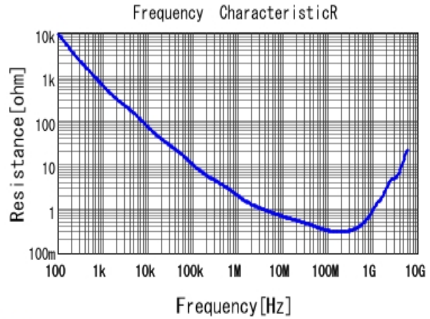
■ GRJ216R72A102KE01 R DCOV, 25degC
