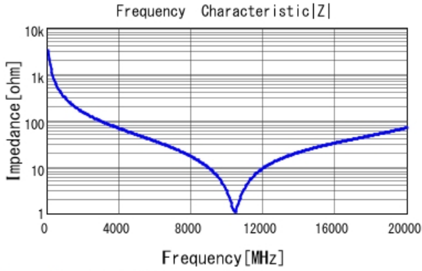
GRM1554C1HR50BA01 |Z| DCOV, 20degC
