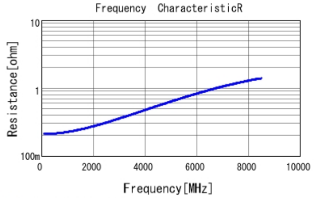
■ GRM0335C2A5R0BA01 R DCOV, 25degC
