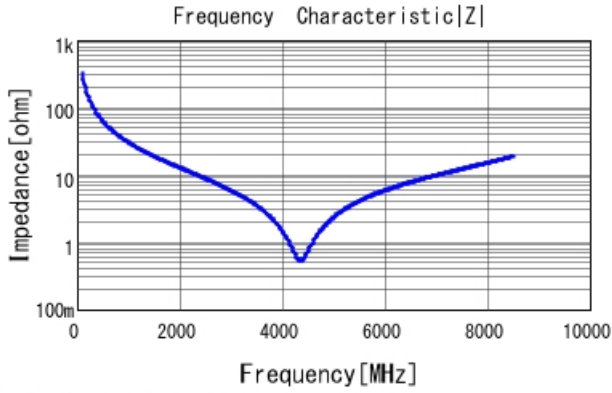
■ GRM0335C2A5R0BA01 |Z| DCOV, 25degC
