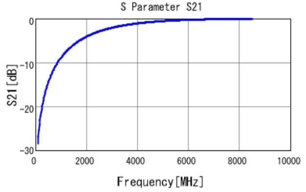
GRM1885C2AR60BA01 S21 DCOV, 25degC
