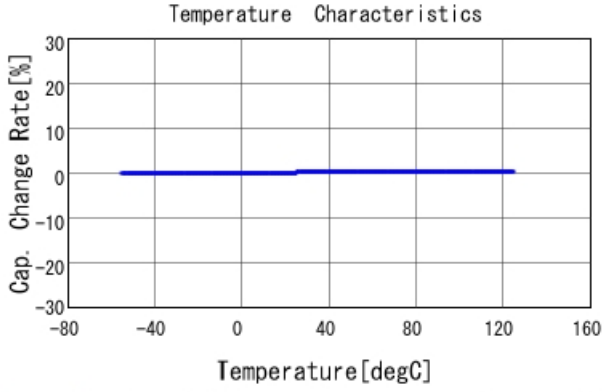
GRM1885C2AR60BA01 C-Temp. capchange, DCOV, AC1Vrms
