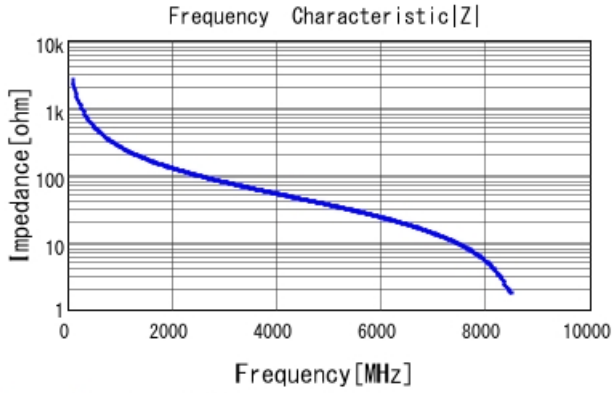
GRM1885C2AR60BA01 |Z| DCOV, 25degC
