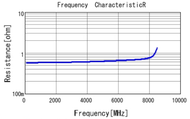
GRM1885C2AR60BA01 R DCOV, 25degC
