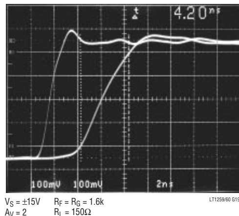
Small-Signal Rise Time
