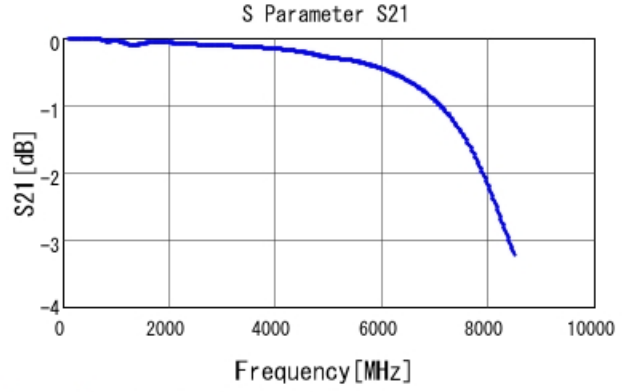
GCM1885C1H331JA16 S21 DCOV, 25degC
