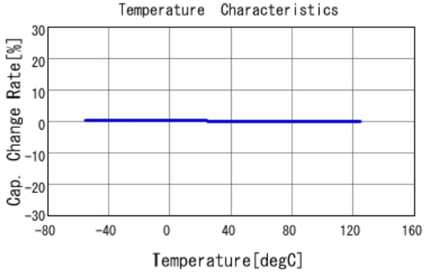
GCM1885C1H331JA16 C-Temp. capchange, DCOV, AC1Vrms
