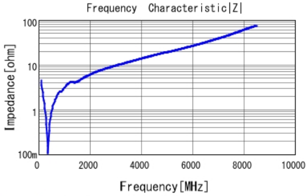
GCM1885C1H331JA16 |Z| DCOV, 25degC
