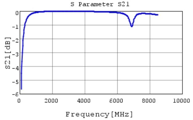
GCQ1555C1H9R7WB01 S21 DCOV, 25degC
