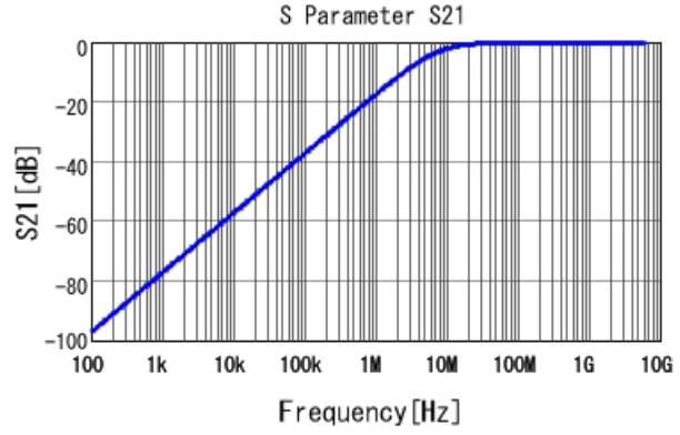
GRM155R71H221KA01 S21 DC0V, 25degC
