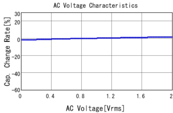
GRM155R71H221KA01 C-AC Voltage capchange, DCOV, 25
