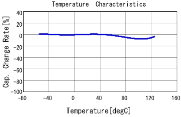
GRM155R71H221KA01 C-Temp. capchange, DC0.0V, AC1.C
