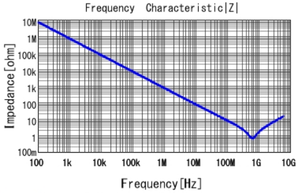
GRM155R71H221KA01 |Z| DCOV, 25degC
