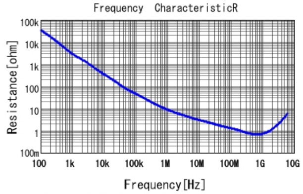
GRM155R71H221KA01 R DCOV, 25degC
