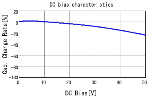
GRM155R71H221KA01 C-DC bias capchange, 25.0degC, A
