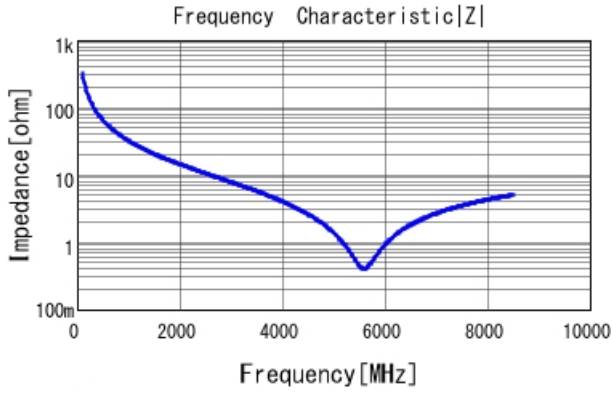
GRM0225C1E4R8WA03 |Z| DCOV, 25degC
