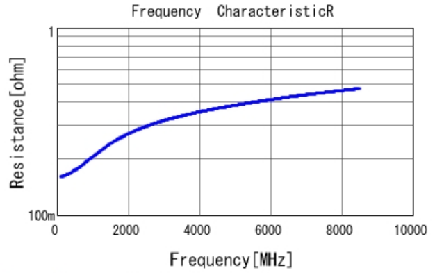
GRM0225C1E4R8WA03 R DCOV, 25degC
