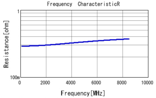
GJM0335C1E1R3WB01 R DCOV, 25degC
