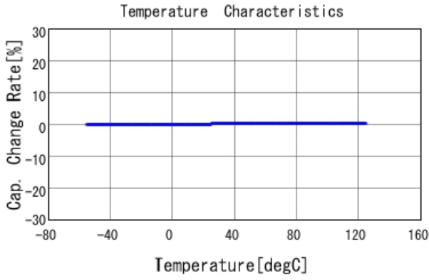
GJM0335C1E1R3WB01 C-Temp. capchange, DC0V, AC1Vrms
