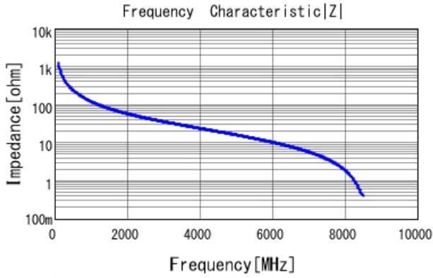
GJM0335C1E1R3WB01 |Z| DCOV, 25degC
