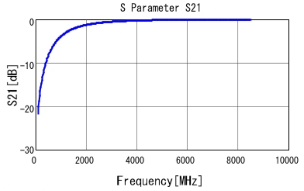
GJM0335C1E1R3WB01 S21 DC0V, 25degC
