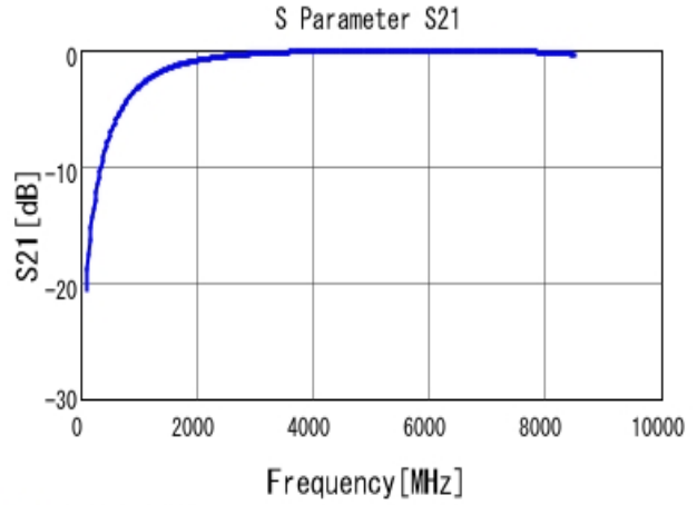
■ GQM1885C2A1R5CB01 S21 DCOV, 25degC
