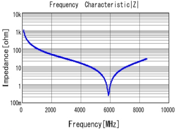
■ GQM1885C2A1R5CB01 |Z| DC0V, 25degC
