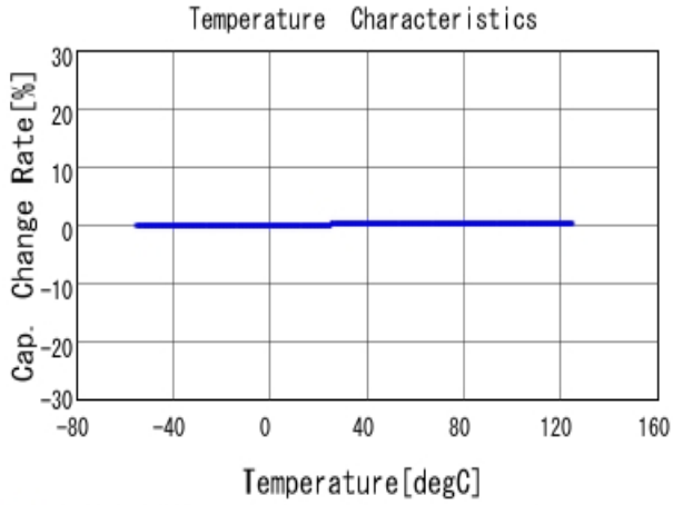
■ GQM1885C2A1R5CB01 C-Temp. capchange, DCOV, AC1Vrms
