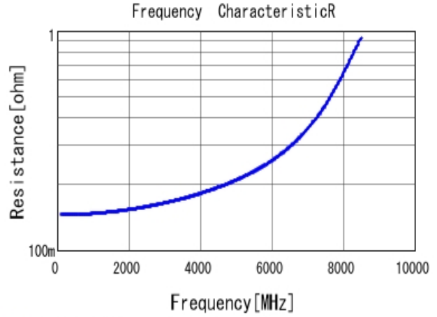
■ GQM1885C2A1R5CB01 R DC0V, 25degC
