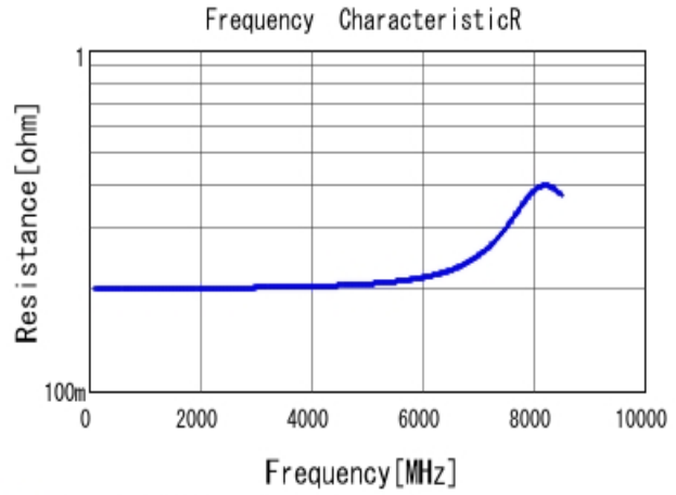
■ GQM2195C2A1R0BB01 R DC0V, 25degC
