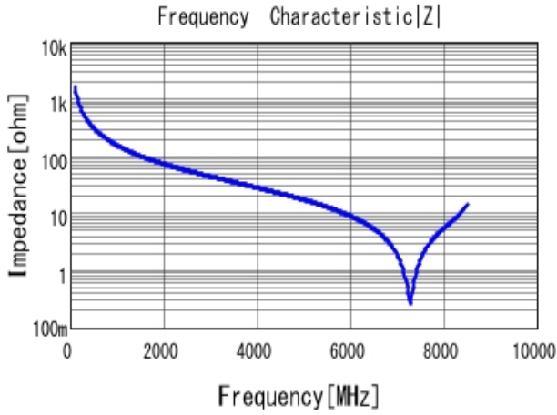
■ GQM2195C2A1R0BB01 |Z| DC0V, 25degC
