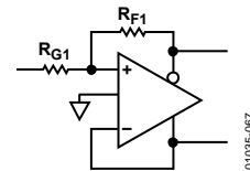
Figure 69. Typical Circuit with \beta_2 = 1
