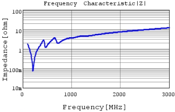
GRM31B5C3A681FWA1 |Z| DC0V, 25degC
