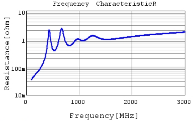
GRM31B5C3A681FWA1 R DC0V, 25degC
