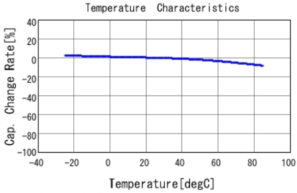
GRM155B11C103KA01 C-Temp. capchange, DC0.0V, AC1.C
