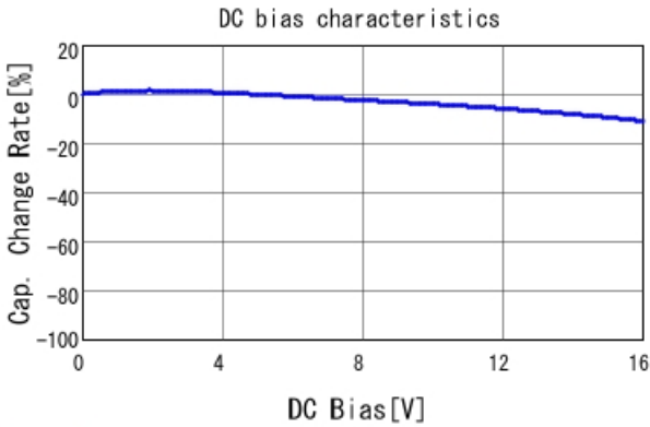
GRM155B11C103KA01 C-DC bias capchange, 20.0degC, A
