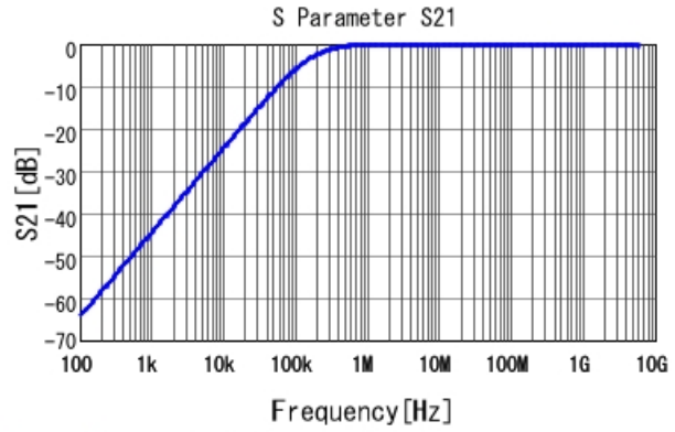
GRM155B11C103KA01 S21 DC0V, 20degC
