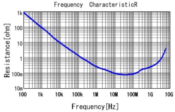
GRM155B11C103KA01 R DCOV, 20degC
