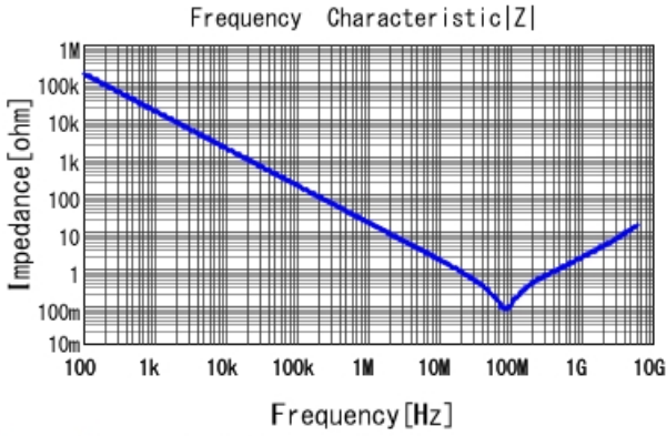
GRM155B11C103KA01 |Z| DCOV, 20degC
