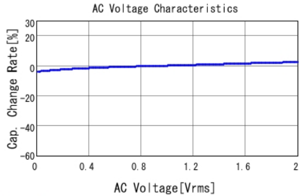
GRM155B11C103KA01 C-AC Voltage capchange, DCOV, 2C
