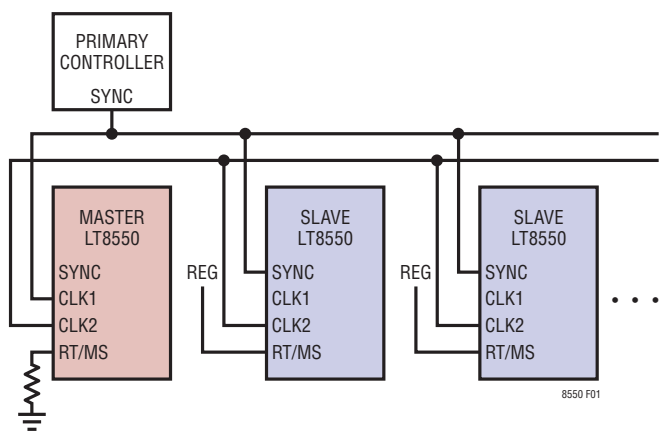
Figure 1. Clock Configuration in a Multiple LT8550 System Table 2 shows the PHS1, PHS2 and PHS3 connections for a two LT8550 system with a total of 9 phases, including the primary controller’s phase, as an example. The
