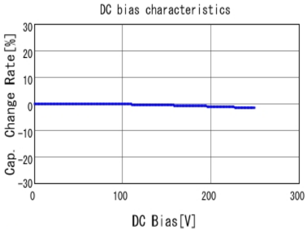
■ GRM32D7U2E473JW31 C-DC bias capchange, 25.0degC, AC1V
