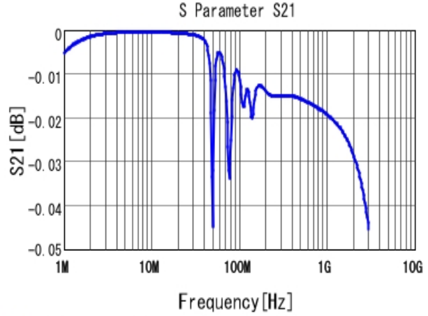
■ GRM32D7U2E473JW31 S21 DCOV, 25degC
