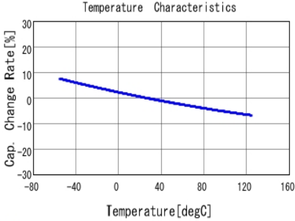
■ GRM32D7U2E473JW31 C-Temp. capchange, DCOV, AC1Vrms
