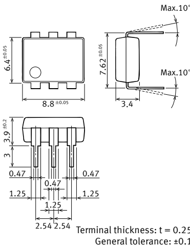
Through hole terminal type External dimensions
