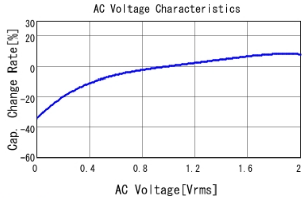
GRM319R6YA106MA12 C-AC Voltage capchange, DCOV, 25
