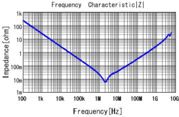
GRM319R6YA106MA12 |Z| DCOV, 25degC
