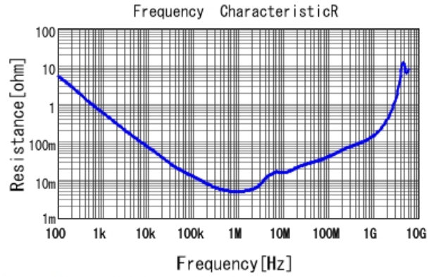
GRM319R6YA106MA12 R DCOV, 25degC
