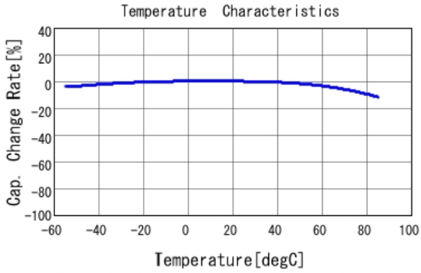
GRM319R6YA106MA12 C-Temp. capchange, DC0.0V, AC1.C
