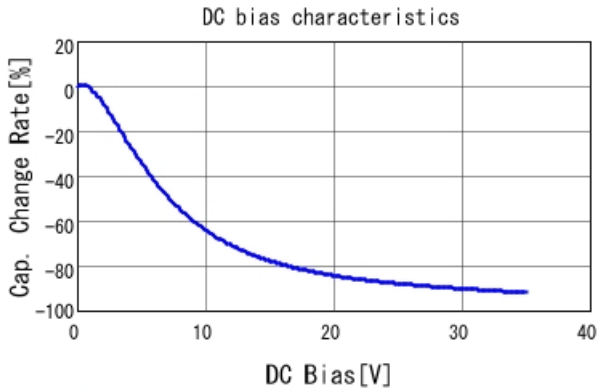
GRM319R6YA106MA12 C-DC bias capchange, 25.0degC, A
