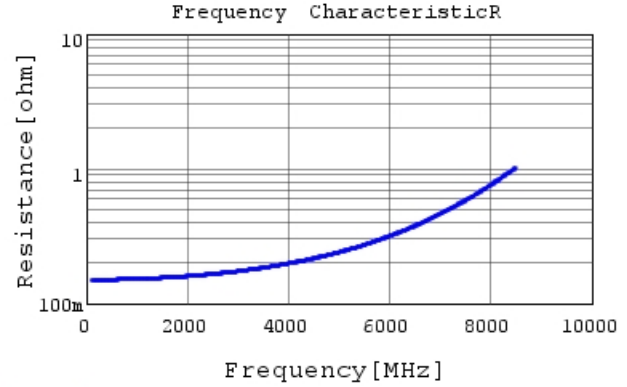
GCQ1555C1H2R5CB01 R DC0V, 25degC
