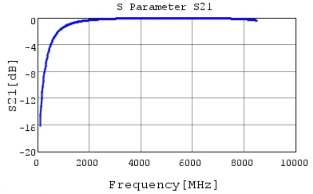
GCQ1555C1H2R5CB01 S21 DC0V, 25degC
