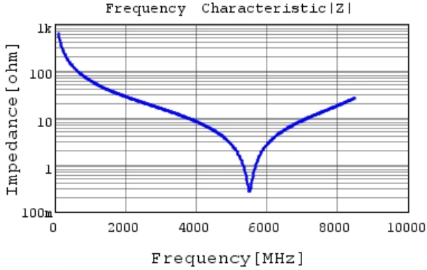
GCQ1555C1H2R5CB01 |Z| DC0V, 25degC
