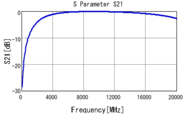
GRM1555C1HR60WA01 S21 DCOV, 25degC
