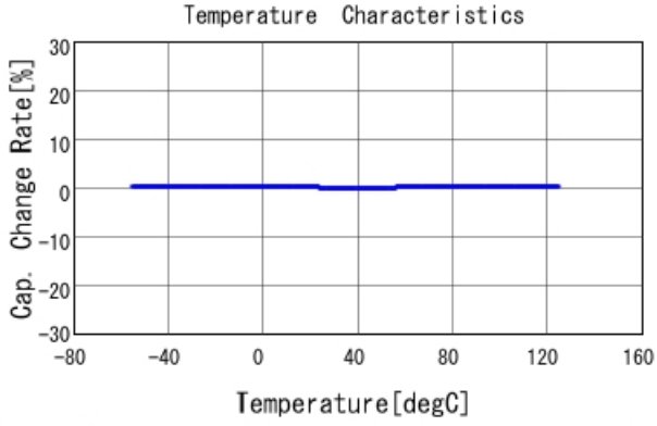
GRM1555C1HR60WA01 C-Temp. capchange, DCOV, AC1Vrms
