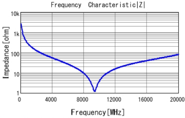
GRM1555C1HR60WA01 |Z| DCOV, 25degC
