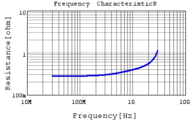
RDE5C1H180J0S1H03A R DCOV, 25degC
