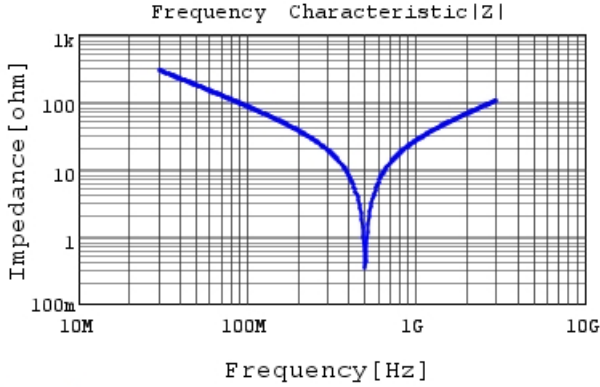
RDE5C1H180J0S1H03A |Z| DCOV, 25degC
