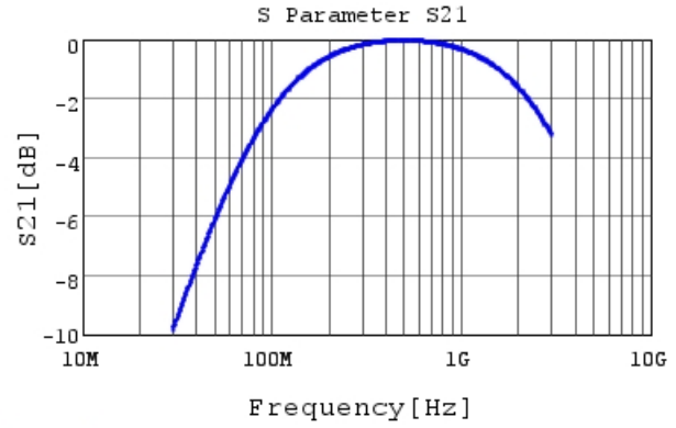
RDE5C1H180J0S1H03A S21 DCOV, 25degC
