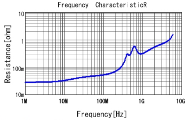
GRM1887U1H122JA01 R DCOV, 25degC
