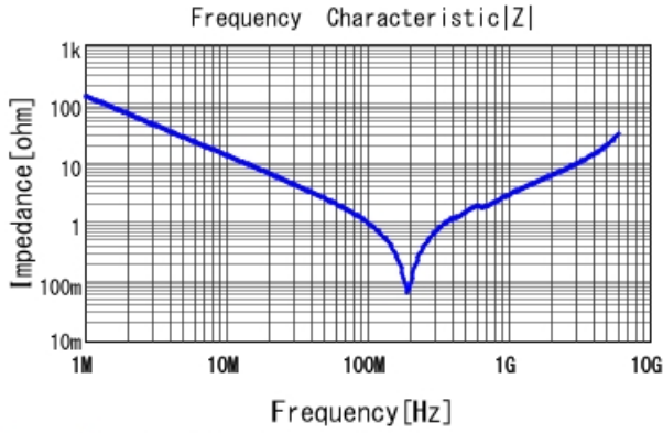
GRM1887U1H122JA01 |Z| DCOV, 25degC
