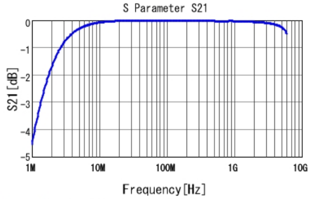
GRM1887U1H122JA01 S21 DCOV, 25degC
