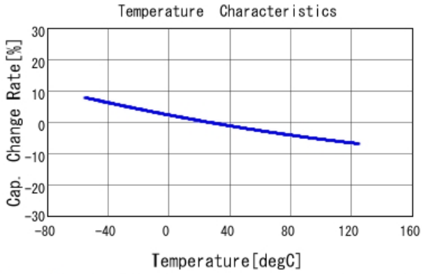
GRM1887U1H122JA01 C-Temp. capchange, DCOV, AC1Vrms
