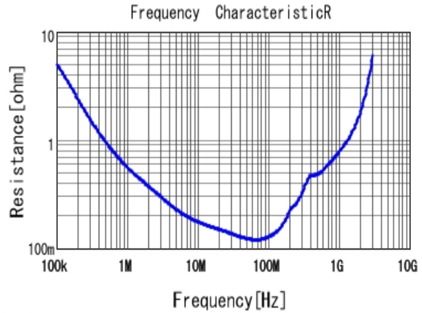
■ GRJ31BR72J472KWJ1 R DCOV, 25degC
