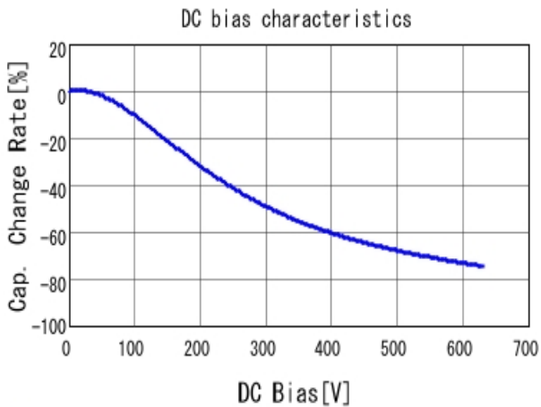
■ GRJ31BR72J472KWJ1 C-DC bias capchange, 25.0degC, AC1V
