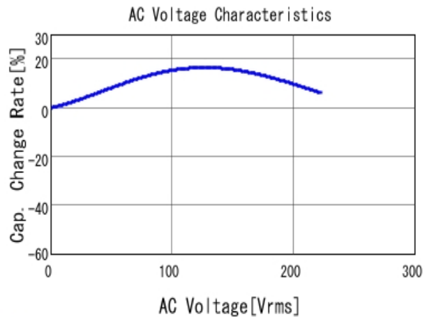
■ GRJ31BR72J472KWJ1 C-AC Voltage capchange, DCOV, 25.0d
