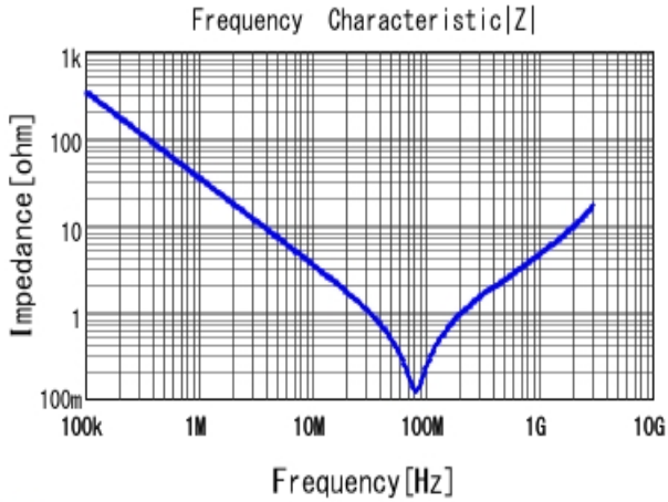
■ GRJ31BR72J472KWJ1 |Z| DCOV, 25degC
