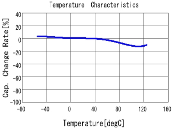
■ GRJ31BR72J472KWJ1 C-Temp. capchange, DCOV, AC1Vrms
