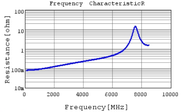
GCQ1555C1H8R5CB01 R DC0V, 25degC
