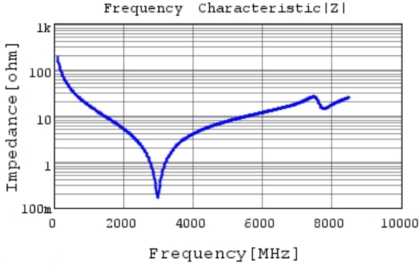
GCQ1555C1H8R5CB01 |Z| DC0V, 25degC
