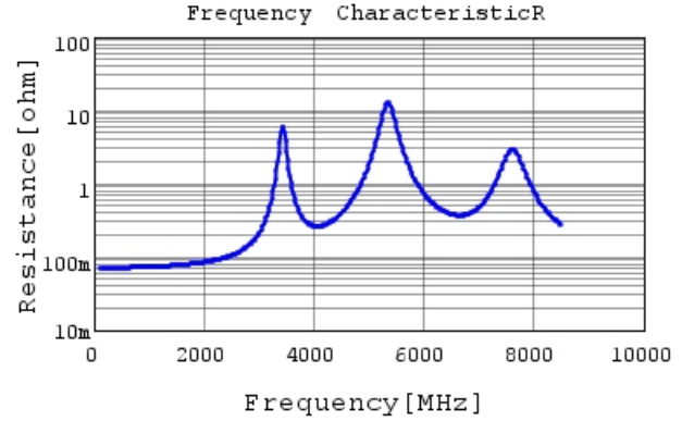
GCQ1555C1H360FB01 R DC0V, 25degC
