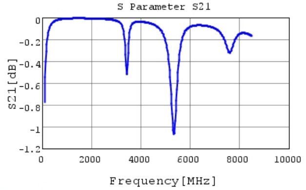
GCQ1555C1H360FB01 S21 DCOV, 25degC
