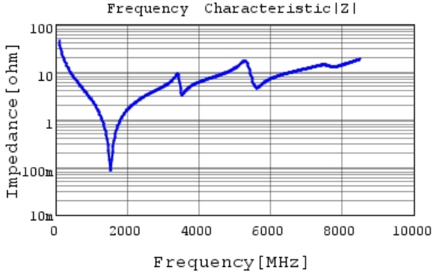
GCQ1555C1H360FB01 |Z| DC0V, 25degC
