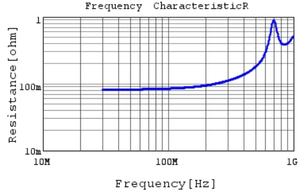
RCE5C2A391J0K1H03B R DC0V, 25degC
