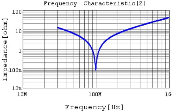
RCE5C2A391J0K1H03B |Z| DC0V, 25degC
