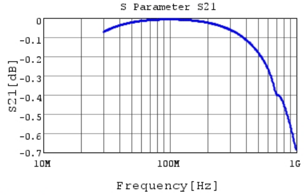
RCE5C2A391J0K1H03B S21 DC0V, 25degC
