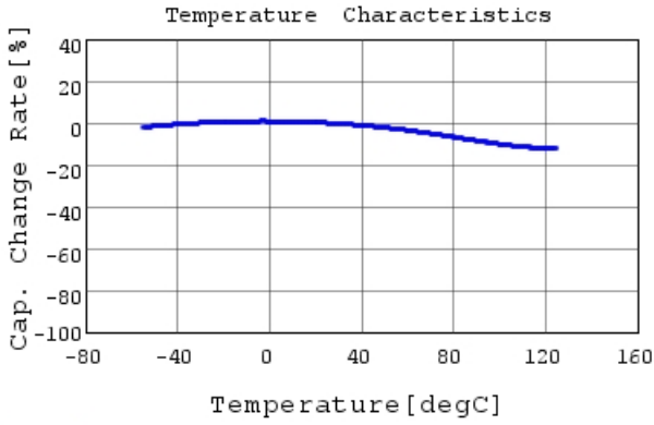
GCM21BR71H474KA55 C-Temp. capchange, DC0.0V,
