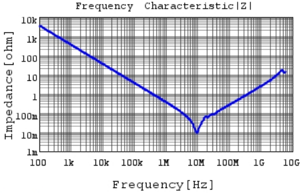
GCM21BR71H474KA55 |Z| DCOV, 25degC
