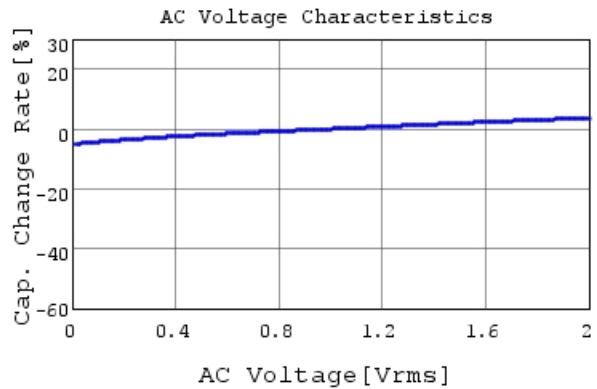
GCM21BR71H474KA55 C-AC Voltage capchange, Dc
