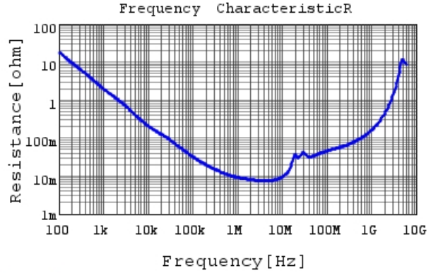
GCM21BR71H474KA55 R DCOV, 25degC
