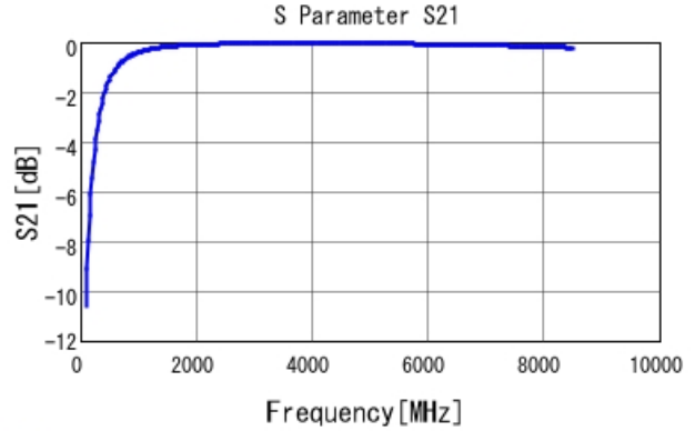
■ GRM0335C2A4R9CA01 S21 DCOV, 25degC
