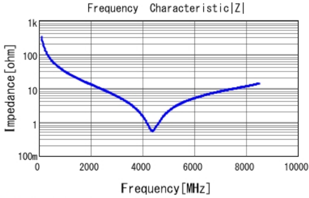
■ GRM0335C2A4R9CA01 |Z| DC0V, 25degC
