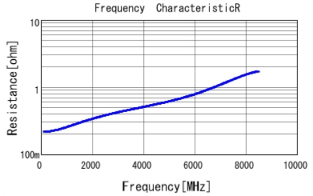
■ GRM0335C2A4R9CA01 R DC0V, 25degC
