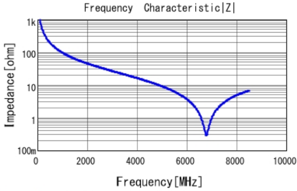
GJM1555C1H1R6BB01 |Z| DCOV, 25degC
