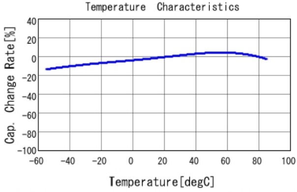
■ GRM033R61A273KE84 C-Temp. capchange, DCO. 0V, ACO. 5Vrm
