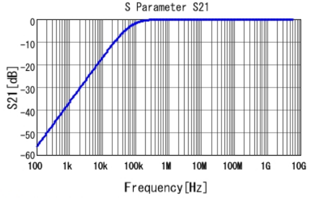
■ GRM033R61A273KE84 S21 DCOV, 25degC
