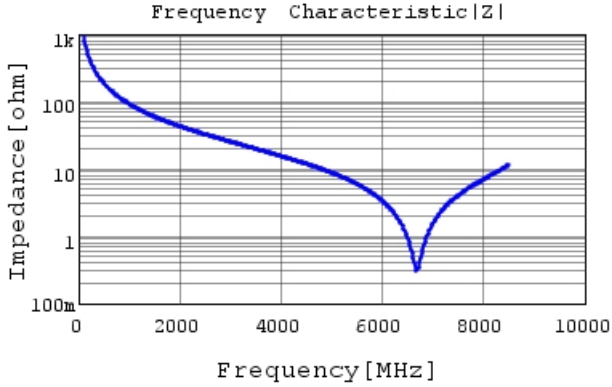
GCQ1555C1H1R7CB01 |Z| DC0V, 25degC
