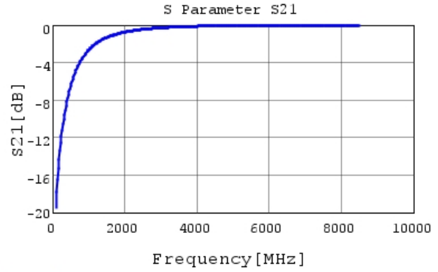
GCQ1555C1H1R7CB01 S21 DCOV, 25degC
