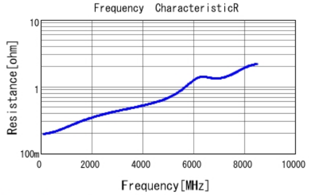
GRM1555C1H8R2BA01 R DCOV, 25degC
