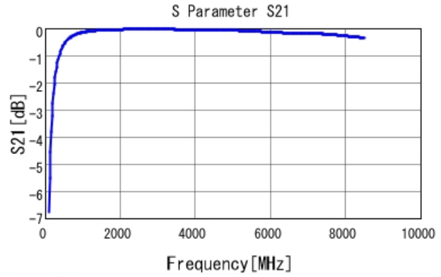
GRM1555C1H8R2BA01 S21 DCOV, 25degC
