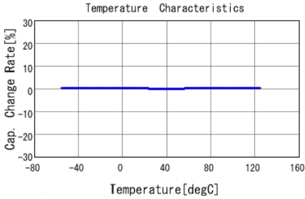
GRM1555C1H8R2BA01 C-Temp. capchange, DCOV, AC1Vrms
