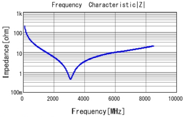
GRM1555C1H8R2BA01 |Z| DCOV, 25degC
