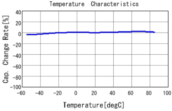
GRM155R61E224KE01 C-Temp. capchange, DC0.0V, AC1.C
