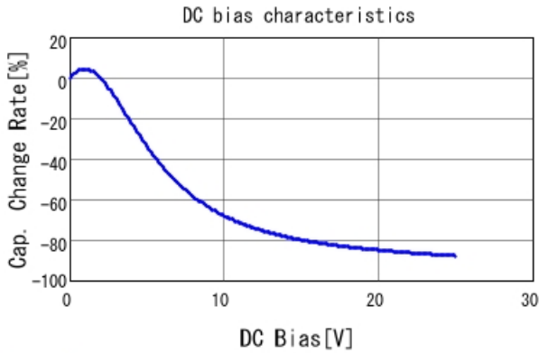
GRM155R61E224KE01 C-DC bias capchange, 25.0degC, A
