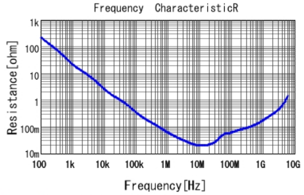
GRM155R61E224KE01 R DCOV, 25degC
