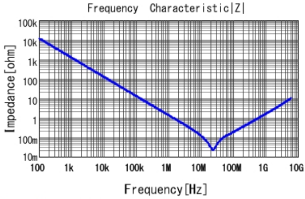
GRM155R61E224KE01 |Z| DCOV, 25degC
